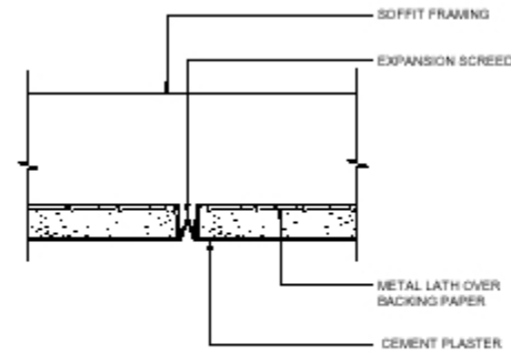
EXPANSION JOINT @ SOFFIT
