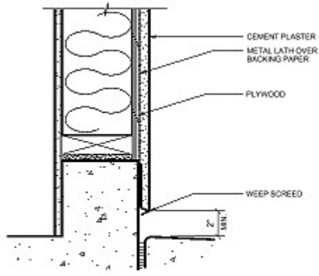
○ FOUNDATION WEEP SCREED
