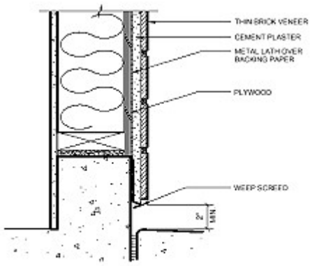
○ FOUNDATION WEEP SCREED
