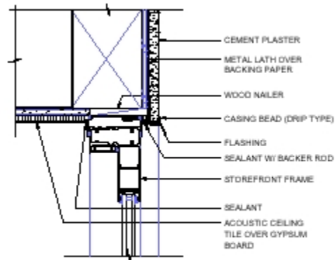
STOREFRONT HEAD
