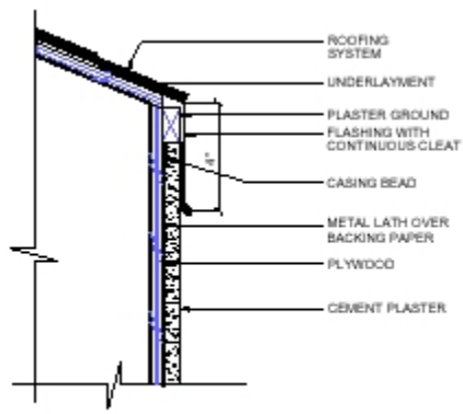
FASCIA
