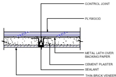
CONTROL JOINT @ THIN BRICK VENEER
