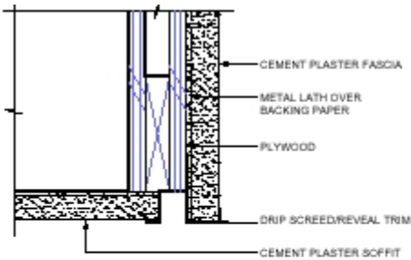
STOREFRONT HEAD
