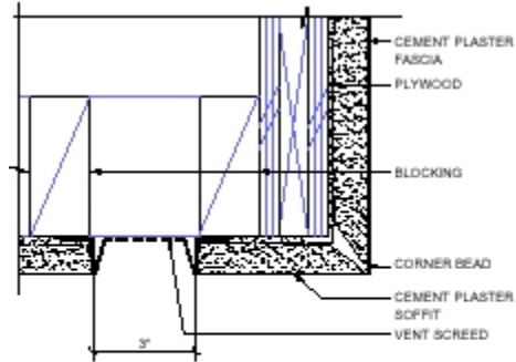
PARAPET CAP @ PLASTER FASCIA
