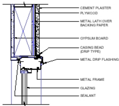
WINDOW HEAD
