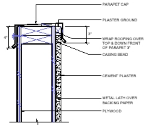
PARAPET CAP @ PLASTER FASCIA
