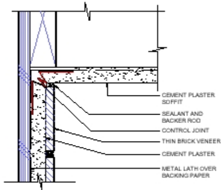
SOFFIT @ WALL-INSIDE CORNER
